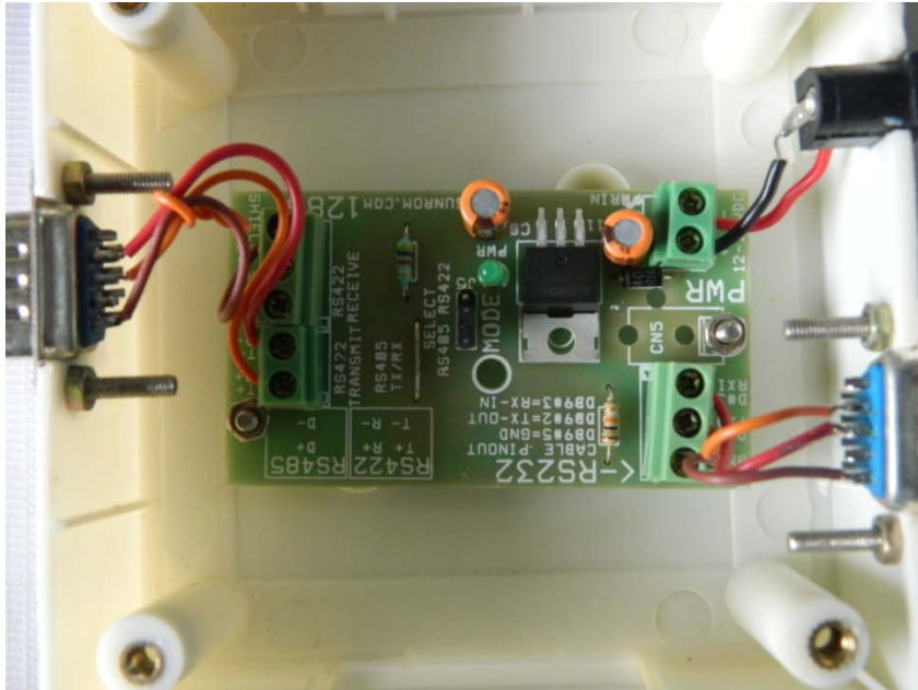
A3: RS 485 to RS 232 converter
