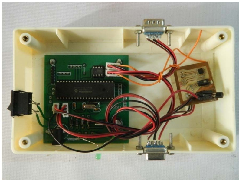
A2: Temperature and RH monitoring sensor node
