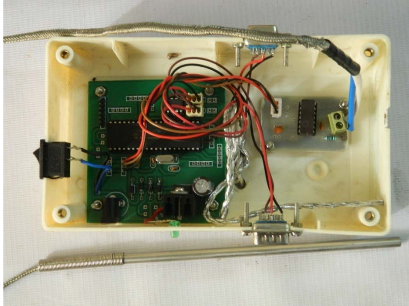
A1: Thermocouple based sensor node
