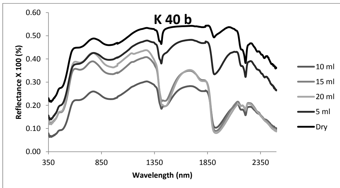
Spectral curve of white soil (K 40 b) with water content variation
