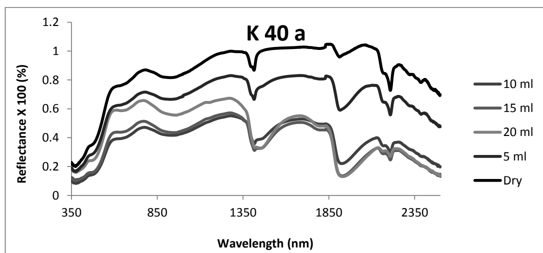
Spectral curve of white soil (K 40 a) with water content variation
