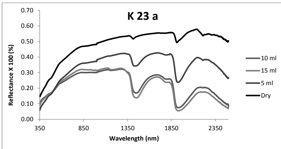
Spectral curve of white soil (K 23 a) with water content variation
