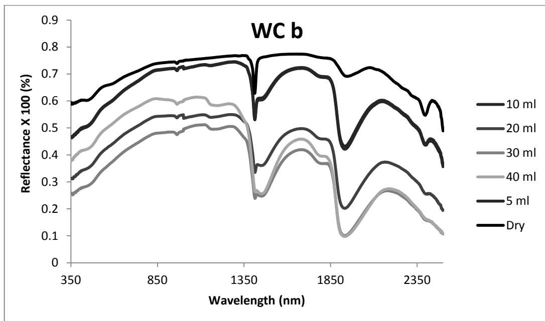
Spectral curve of white soil (WC b) with water content variation
