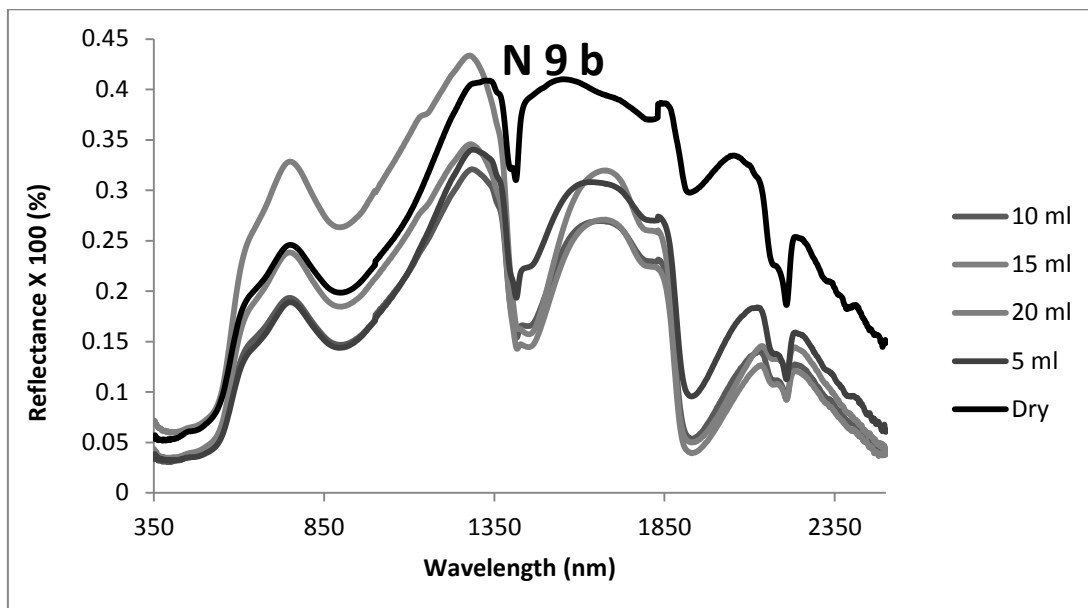
Spectral curve of red soil (N 9 b) with water content variation
