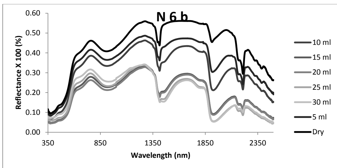
Spectral curve of red soil (N 6 b) with water content variation
