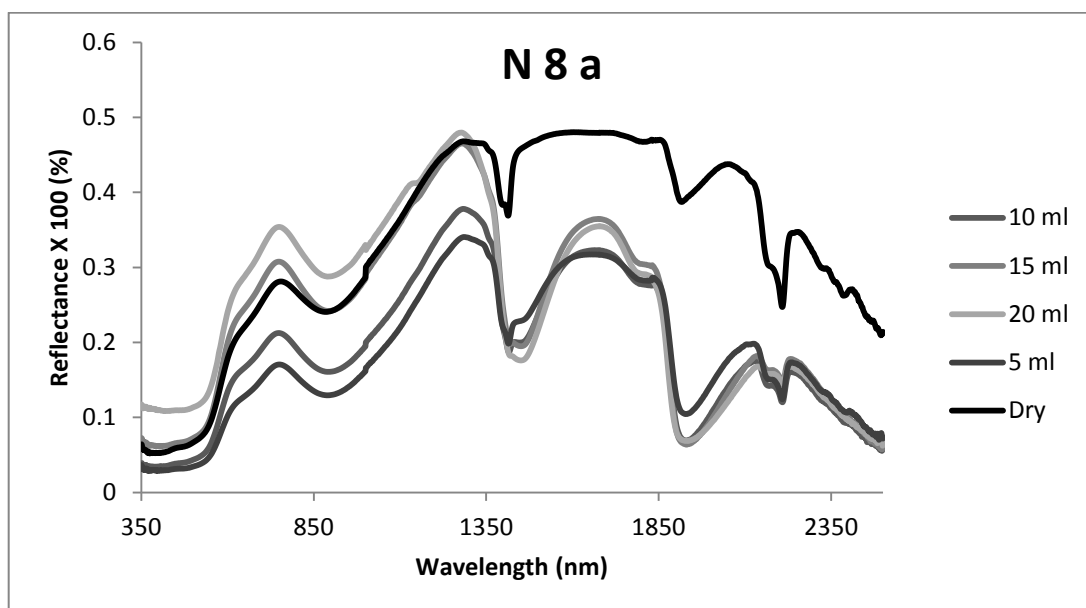
Spectral curve of red soil (N 8 a) with water content variation
