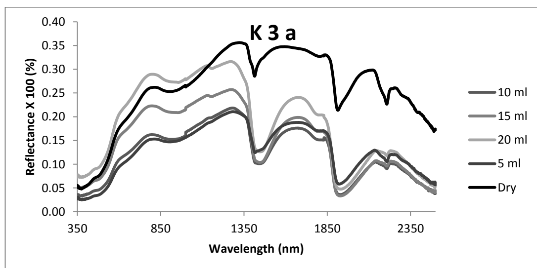
Spectral curve of red soil (K 3 a) with water content variation
