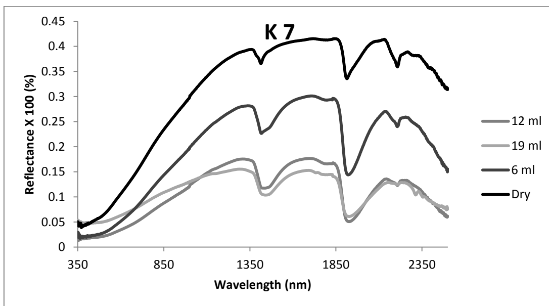
Spectral curve of black soil (K 7) with water content variation
