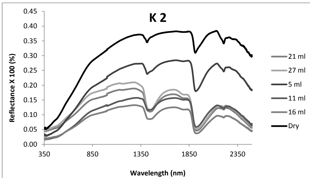
Spectral curve of black soil (K 2) with water content variation
