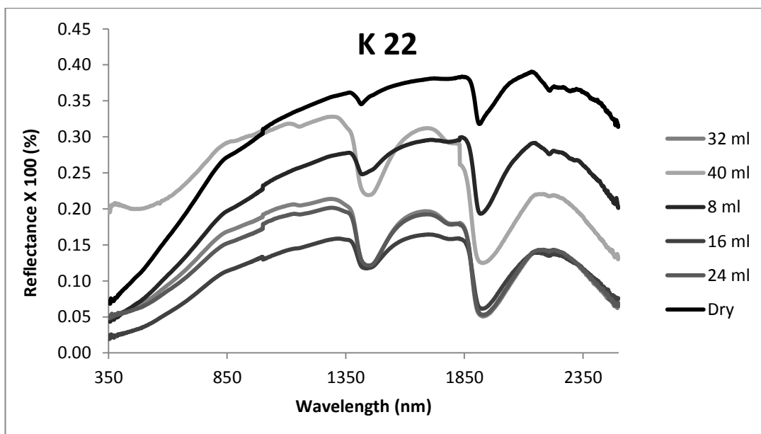
Spectral curve of black soil (K 22) with water content variation
