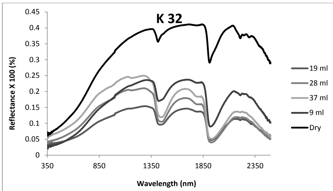
Spectral curve of black soil (K 32) with water content variation
