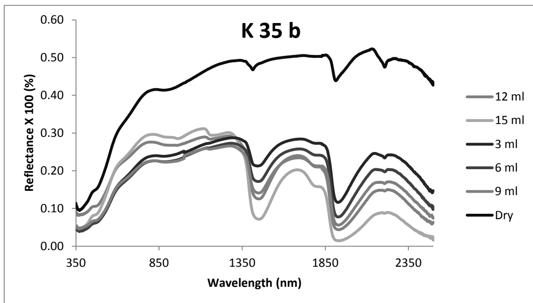
Spectral curve of brown soil (K 35 b) with water content variation
