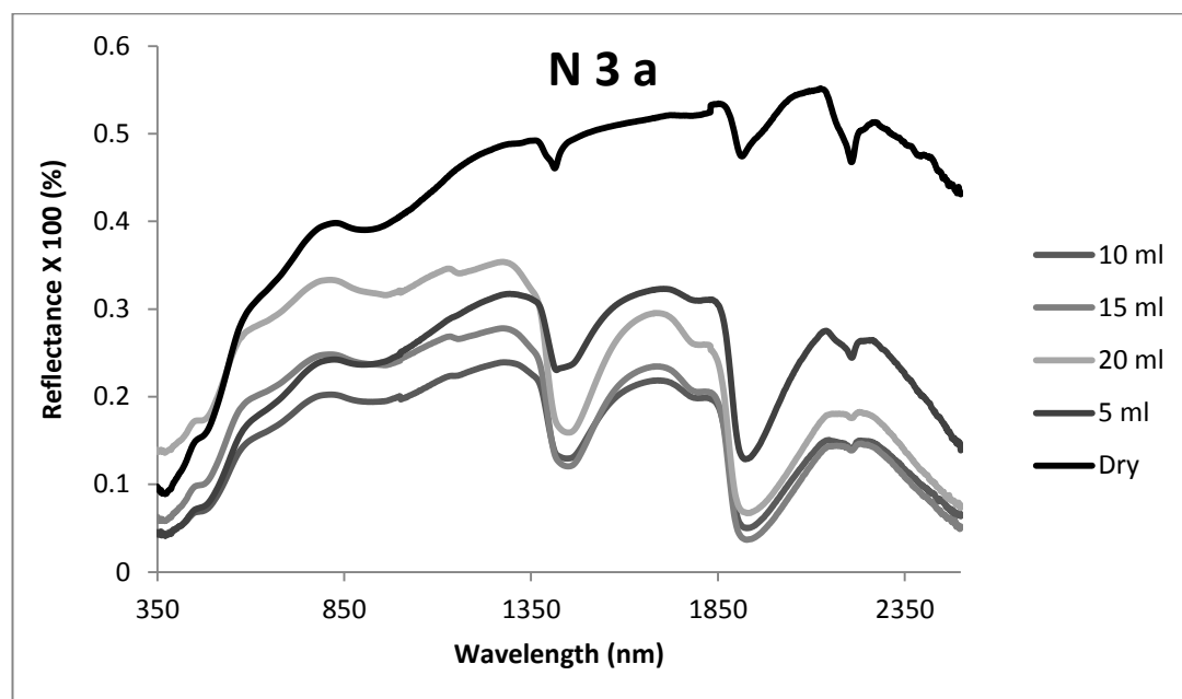
Spectral curve of brown soil (N 3 a) with water content variation
