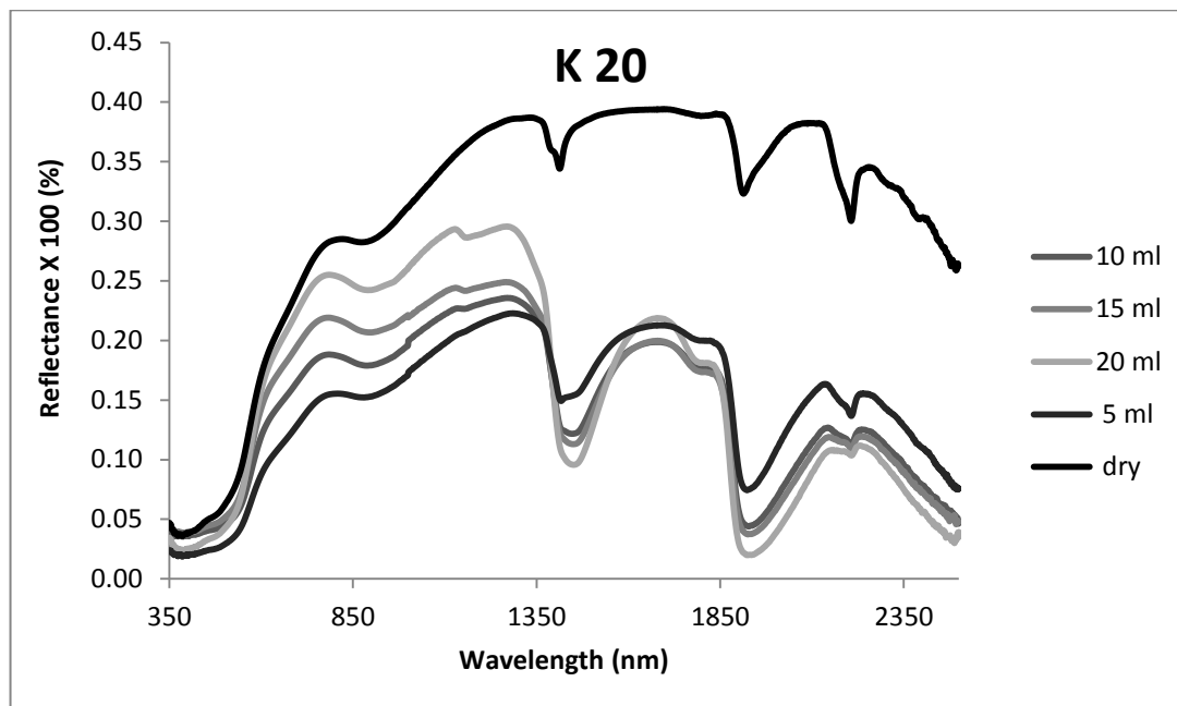
Spectral curve of brown soil (K 20) with water content variation
