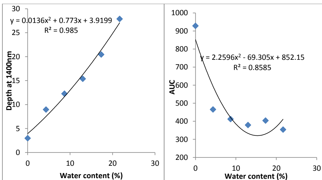
Relationship between Water content and Spectral parameters of sample K 35 b
