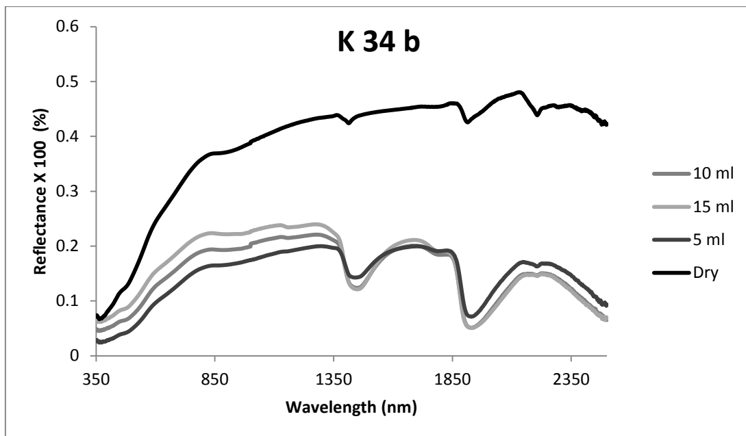
Spectral curve of brown soil (K 34 b) with water content variation
