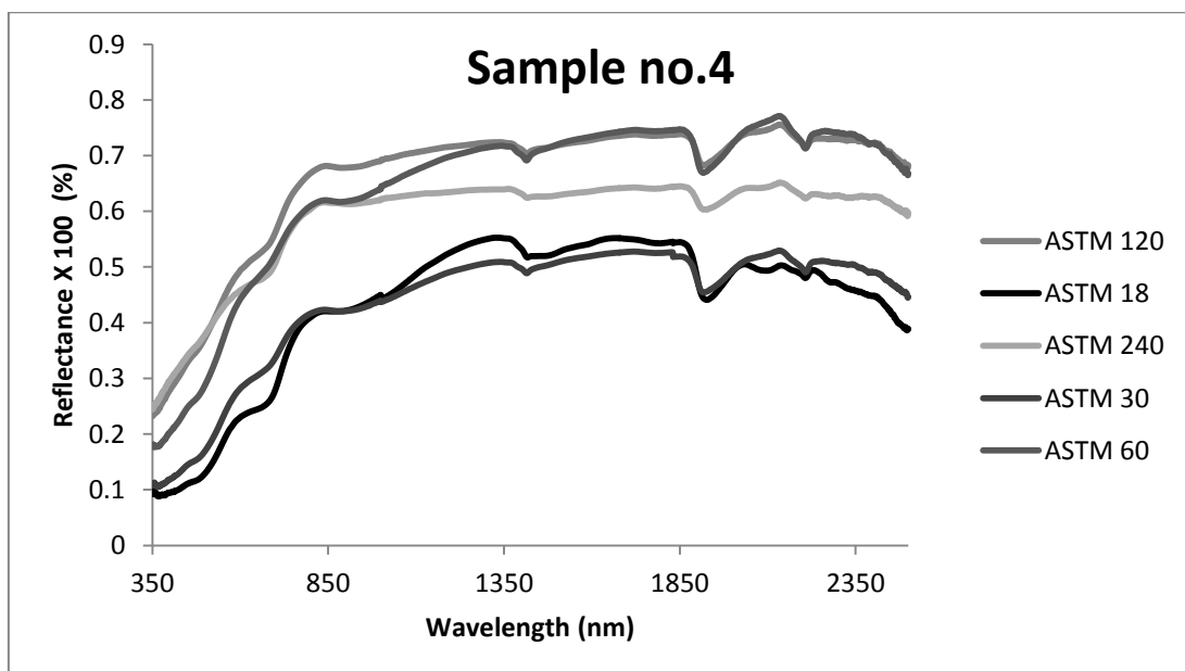
Spectral curve of river sand (Sample no.4) with texture variation
