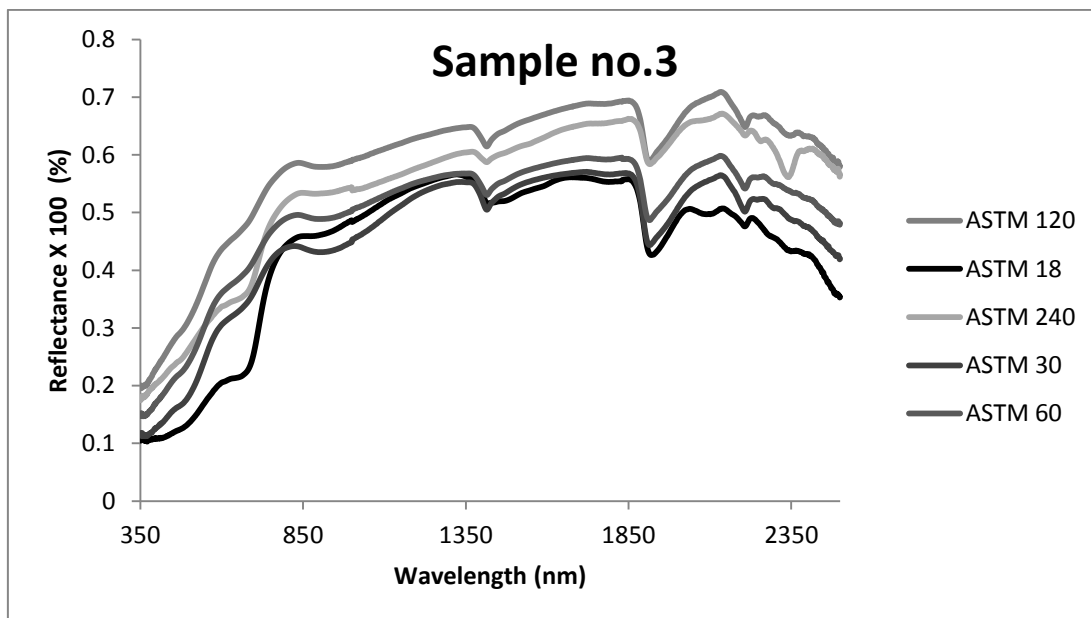
Spectral curve of river sand (Sample no.3) with texture variation
