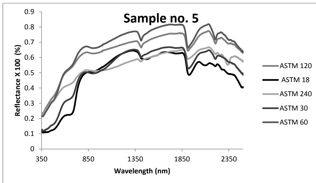
Spectral curve of river sand (Sample no.5) with texture variation
