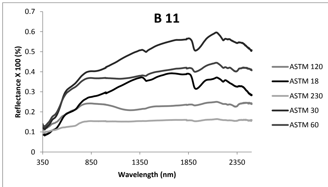
Spectral curve of beach sand (B 11) with texture variation
