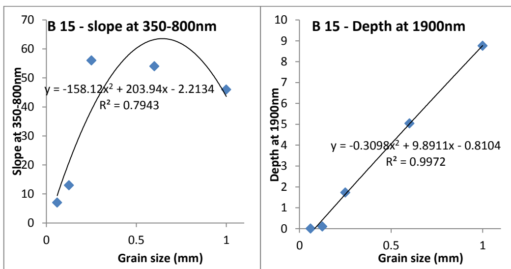
Relationship between grain size and Spectral parameters of sample B 15
