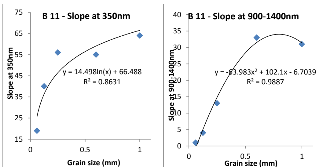
Relationship between grain size and Spectral parameters of sample B 11
