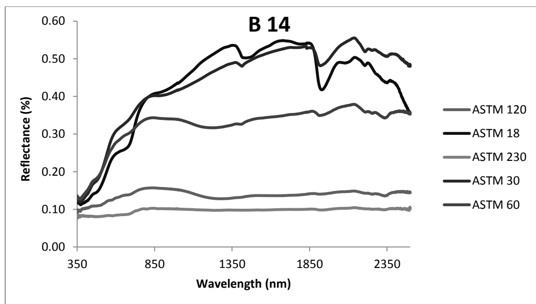
Spectral curve of beach sand (B 14) with texture variation
