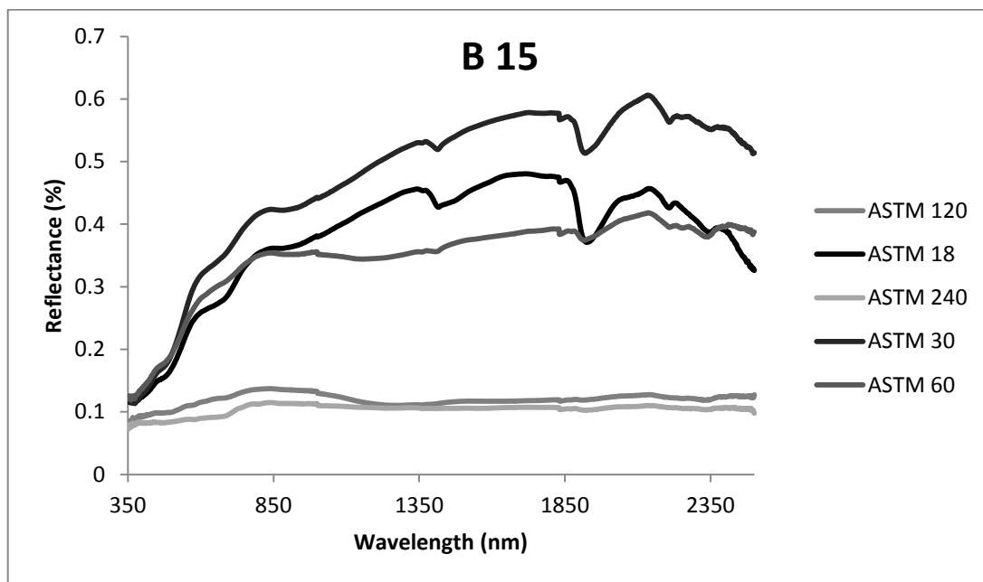
Spectral curve of beach sand (B 15) with texture variation
